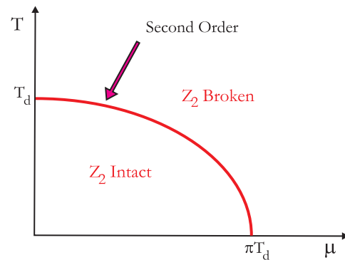
FIG. 3: A schematic (T, \mu) -phase diagram where only deconfinement is considered
