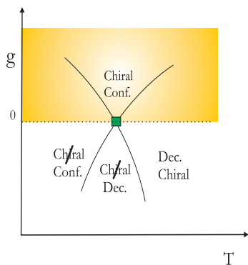
FIG. 1: Phase diagram displaying a tetracritical point. The physically allowed part of the phase diagram lies beneath the g = 0 line.
