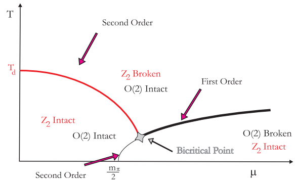
FIG. 5: A possible (T, \mu) -phase diagram when both possible phase transitions, chiral and confinement, are taken into account and meet at a bicritical point.
