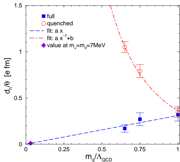
Fig. 3: ILM results obtained at different values of the quark masses with quenched (circles) and unquenched (squares) simulations. The behavior of the unquenched and quenched calculations for small quark masses is consistent with Eqs. (4.9) and (4.10), respectively.
