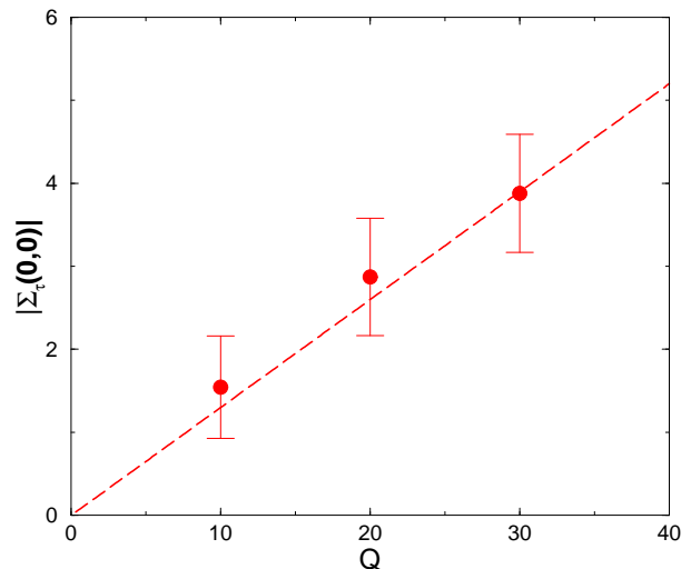
Fig. 2: Absolute value of the correlation function \tilde{\Sigma}_\tau(\mathbf{0}, \mathbf{0}) as a function of the topological charge Q . Notice that the correlator (2.13), which relates directly to the EDM, receives contributions only from topologically non-trivial sectors, as expected. These results were obtained in the quenched approximation, by averaging over the configurations of an ensemble of 130 pseudo-particles in a volume V = 3.1^3 \times 4 = 120 fm 4 and quark masses of m_q = 0.65 \Lambda_{QCD} .
