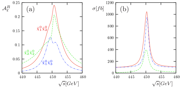
Figure 5: \mu^+\mu^- \rightarrow \tilde{\chi}_i^0\tilde{\chi}_j^0 , \tilde{\chi}_j^0 \rightarrow \ell^-\tilde{\ell}_R^+ , \ell = e, \mu , for scenario B10 with i = 1, j = 2 (solid), i = 1, j = 3 (dash-dotted) and i = 2, j = 2 (dashed). (a): \mathcal{A}_\ell^R and (b): neutralino production cross section, with P_+^L = P_-^L = -0.3 .
