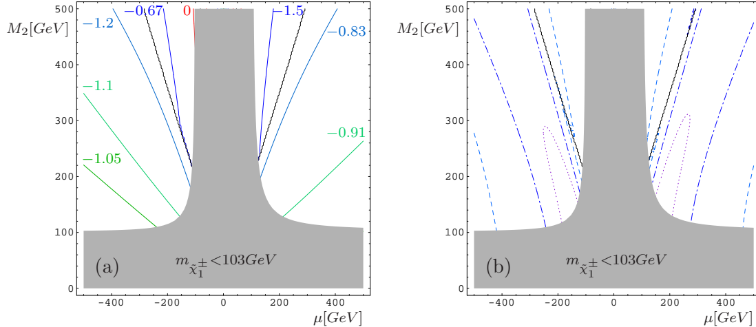
Figure 6: Contours of constant \gamma_{12}r_{12} (a) and \text{Im}(c_{ij}^{(H)}c_{ij}^{(A)*}) (b), for \tan\beta = 10 and m_A = 450 GeV. In (b) we show \text{Im}(c_{ij}^{(H)}c_{ij}^{(A)*}) = 0.01 (dashed), 0.03 (dash-dotted) and 0.05 (dotted). The wiggly lines in both figures indicate the level crossing of the \tilde{\chi}_2^0 and \tilde{\chi}_3^0 states, with \eta_{12} = 1 in the area below and \eta_{12} = -1 in the area above the level crossing line. The gray area is experimentally excluded by m_{\tilde{\chi}_1^\pm} < 103 GeV.
