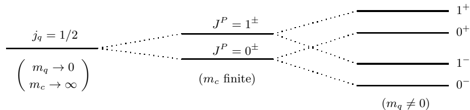
FIGURE 2: Procedure how the degeneracy is resolved in [2].
