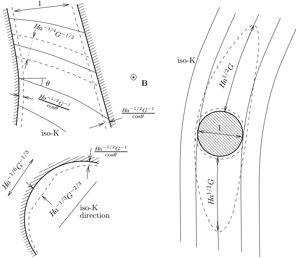
FIGURE 4. Two-dimensional MHD structures.
