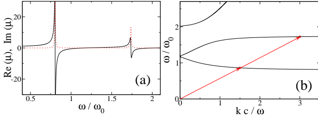
FIG. 2: (a) Real (solid) and imaginary (dashed) parts of magnetic permeability of the binary metamaterial. (b) Spectrum of electromagnetic waves. Arrows show the perfectly phase-matched second-harmonic generation.
